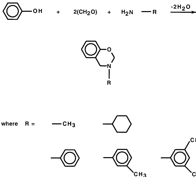
Scheme 1 Monomer synthesis.
